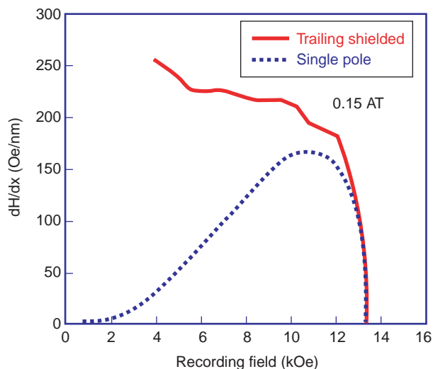
Figure 12 Recording field gradient.
