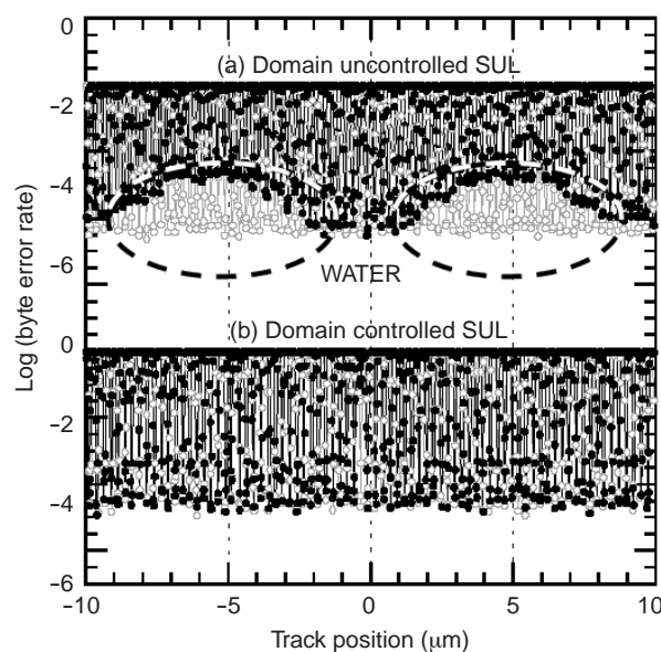
Figure 4 Initial (gray circles) and post erasure (black circles) WATER characteristic of PMR media with (a) domain uncontrolled and (b) controlled SUL.
