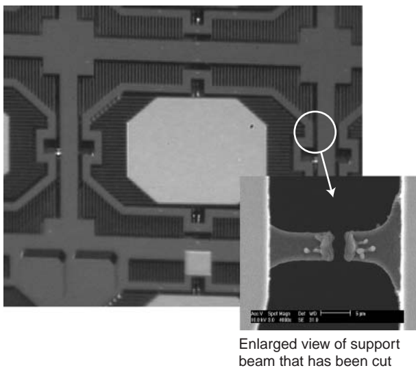
Figure 4 Laser cutting of support beam in MEMS device.
