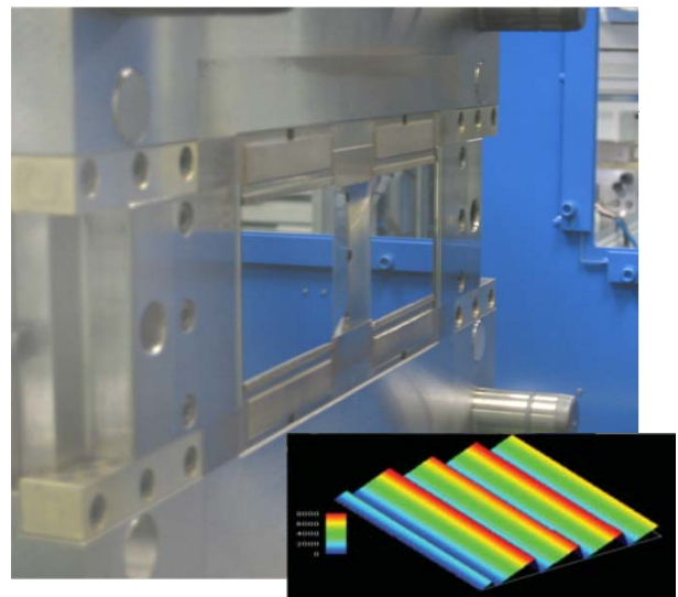
Figure 5 Appearance and prism pattern of metal mold for molding backlight guide plate.
