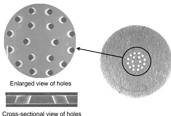
Figure 7 Automobile fuel injection nozzle plate.
