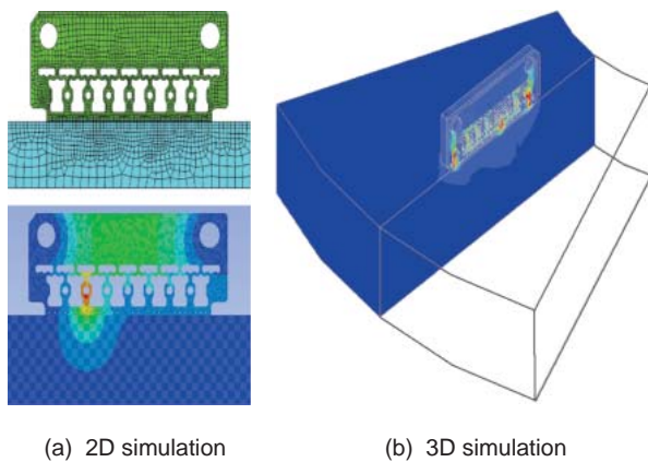
Figure 2 Simulation of lap rates.
