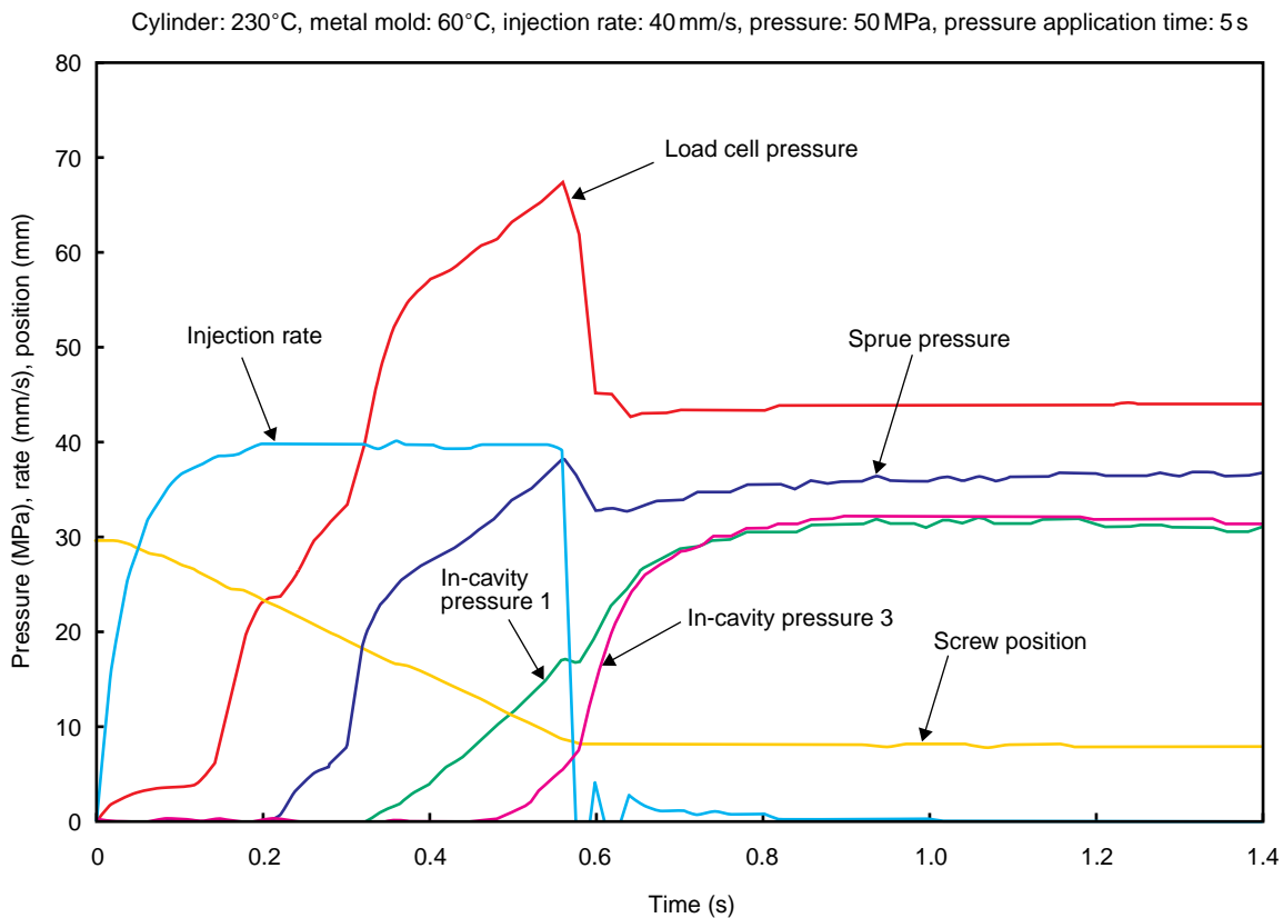
Figure 6 Monitoring of injection molding process.
