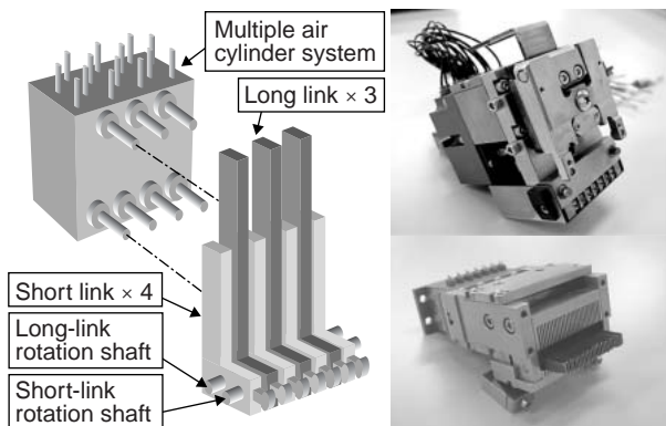
Figure 1 Structure of multi-point actuator.
