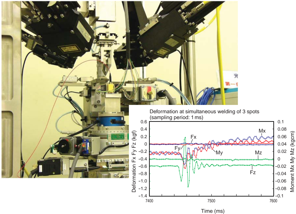
Figure 3 In-process monitoring of deformation at laser welding.
